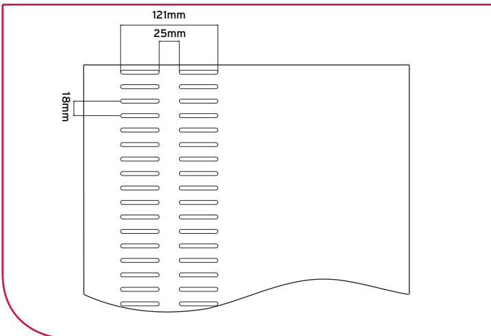
Twice the amount of Slots as the GPB, this means superior Ventilation
